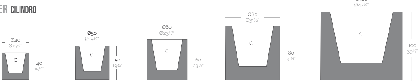
Cylinder Ø15¼" Cilindro Ø40 cm Cylinder Ø19¾" Cilindro Ø50 cm Cylinder Ø23½" Cilindro Ø60 cm Cylinder Ø31½" Cilindro Ø80 cm Cylinder Ø47¼" Cilindro Ø120 cm
